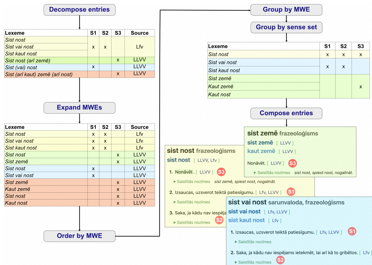
Figure 2: Processing of MWEs with overlapping data
