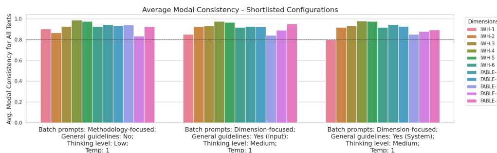
Figure 2: Average modal consistency comparison between the three shortlisted configurations.
